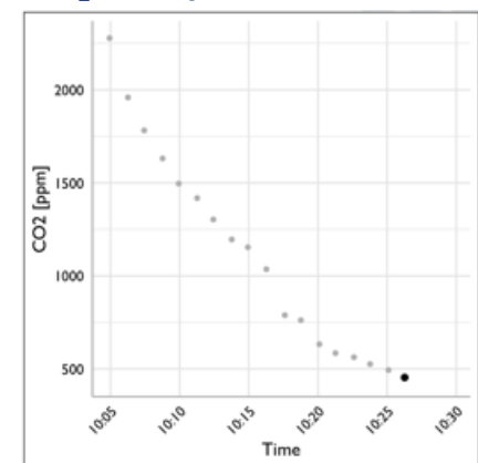
CO 2 Decay
